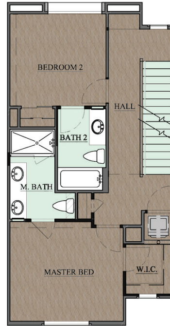
Plan 1a: Third Floor
